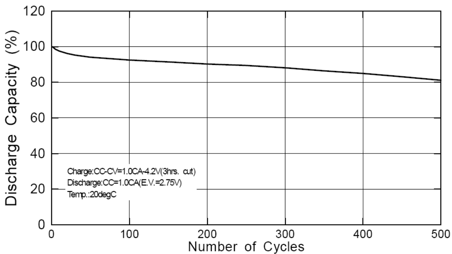
Fig.3-11: Cycle Characteristics
